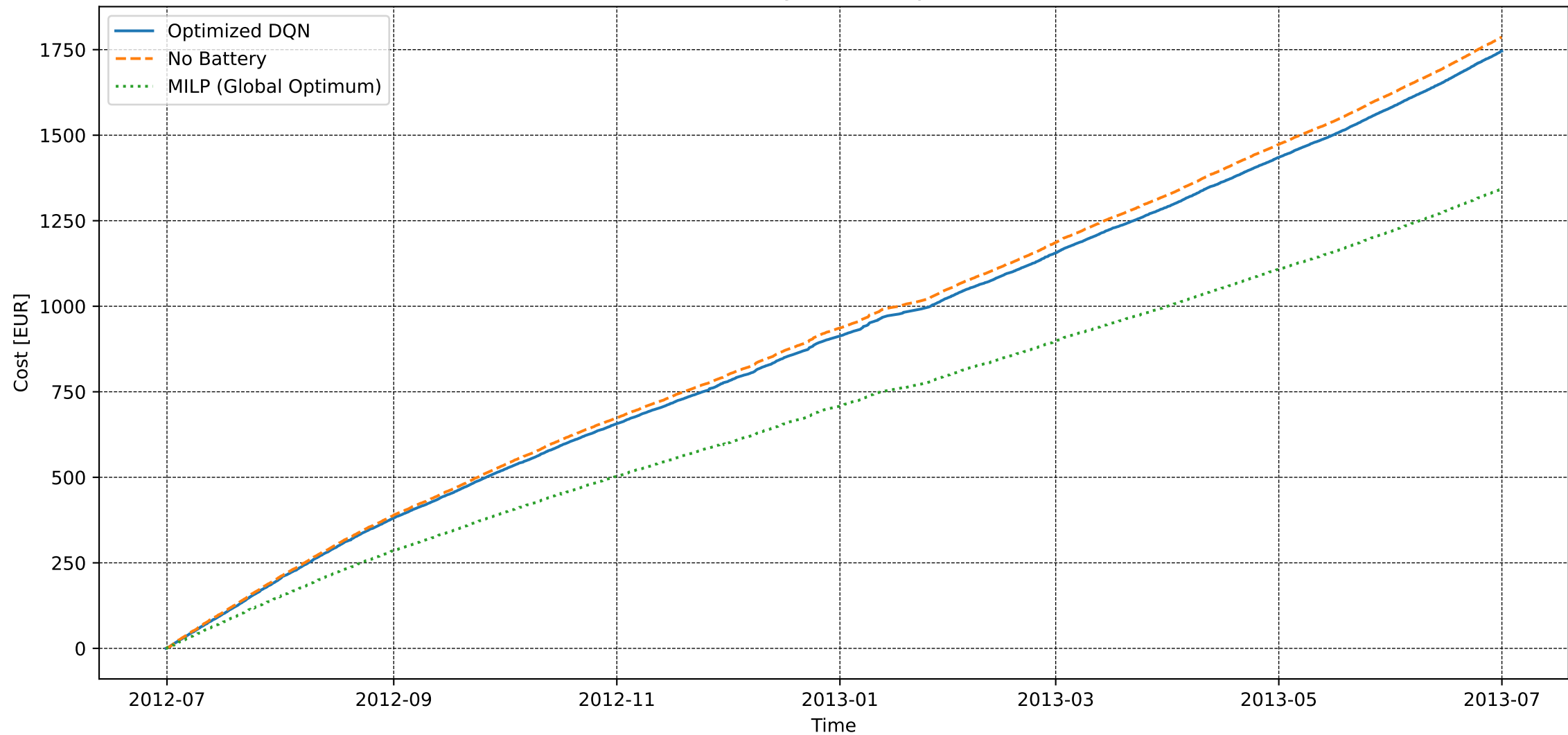
User 156 - Basic Training - Electricity Cost [DQN vs MILP]
